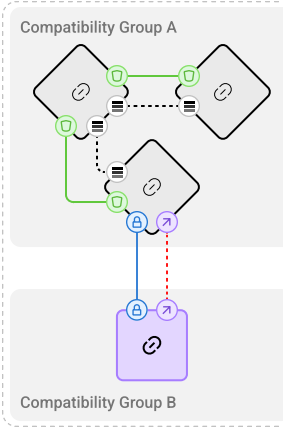
Figure 1: The omnichain fully-connected mesh network has universal network semantics for all connected chains and security specialized to each link.
